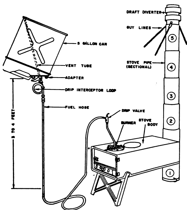
2 Installation setup
