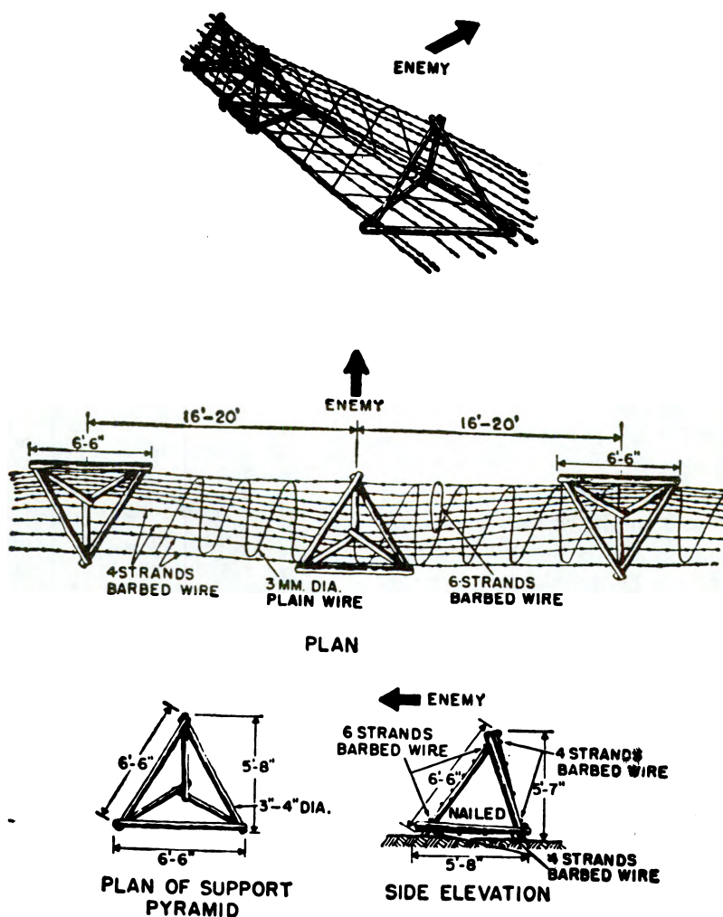
Figure 6-37. Lapland barbed wire.
