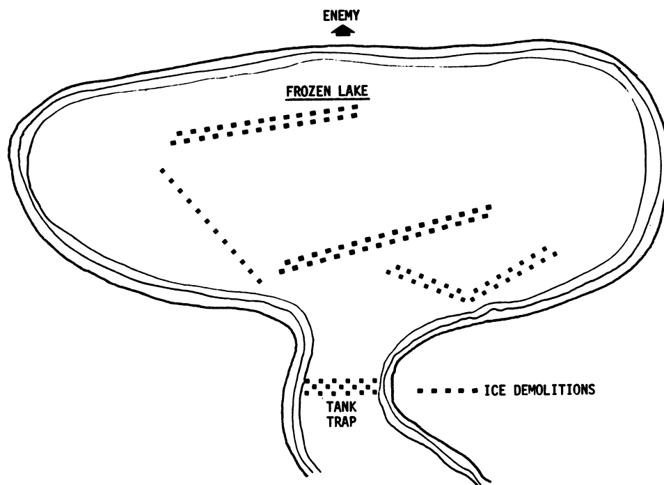
Figure 6-36. Ice demolitions.
