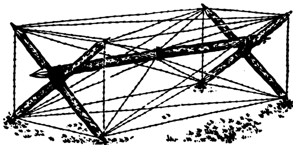
Figure 6-38. Knife rest.
