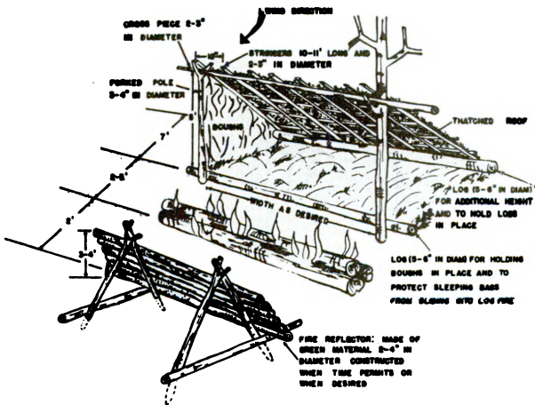
Figure 3-10. Single lean-to.
