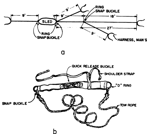
Figure 4-36. Modified tandem system.
