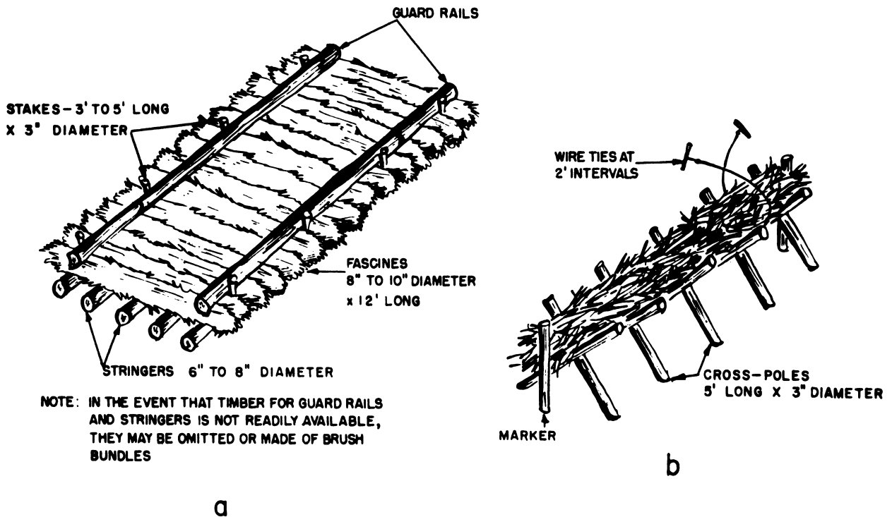
Figure 5-11. Types of corduroy roads.
