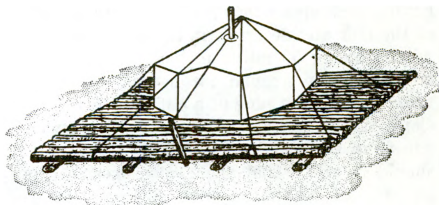
Figure 3-21. "Float" under shelter.
