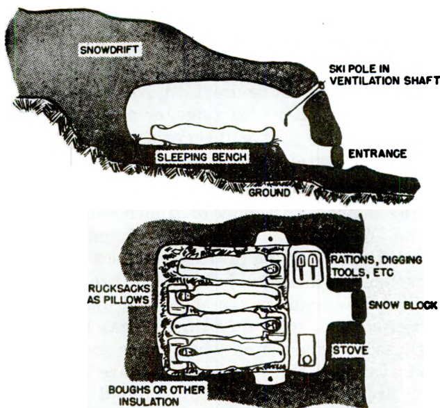
Figure 3-15. Snow cave for four men.
