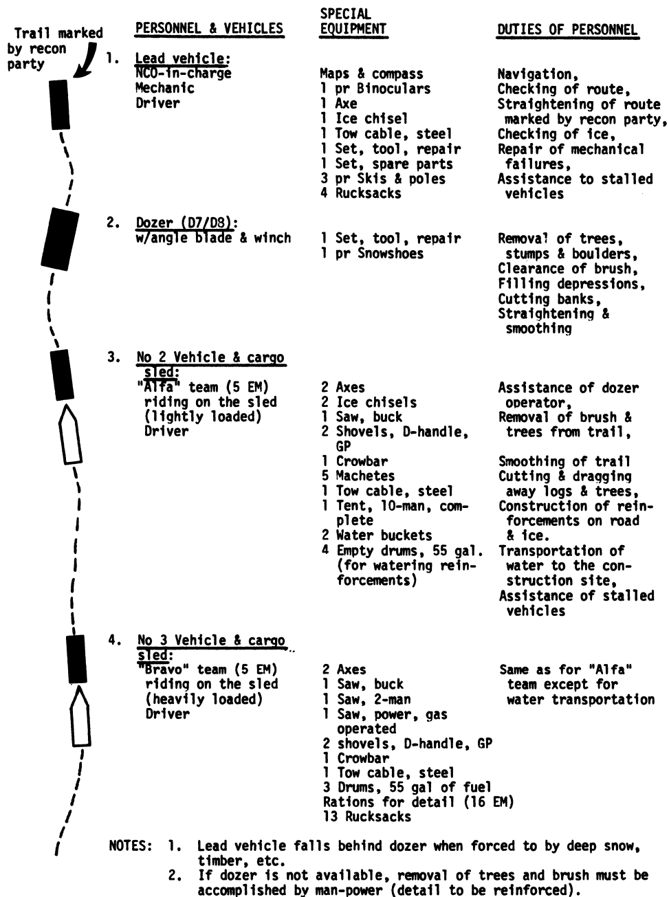
Figure 5-6. Construction detail for winter roads.
