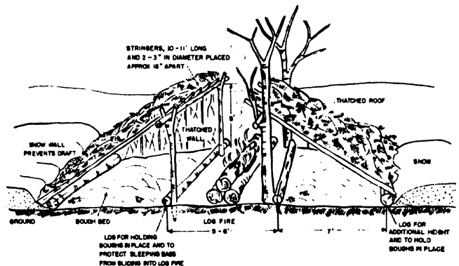
Figure 3-11. Double lean-to.
