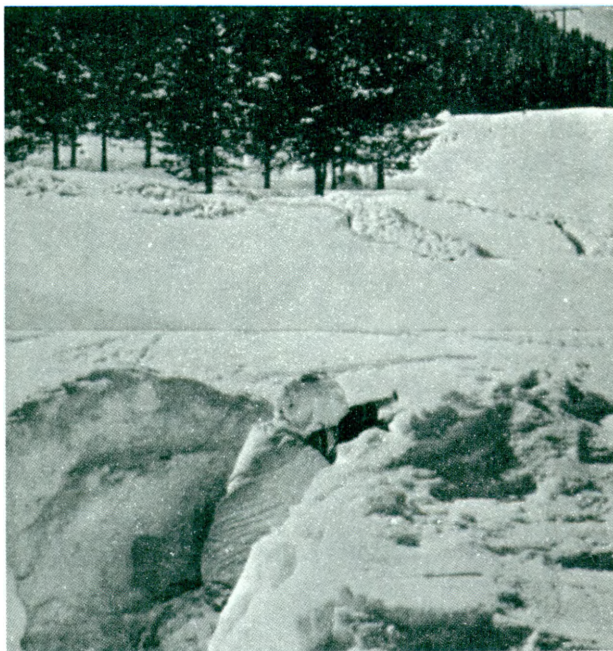
Figure 6-23. Snow trenches.
