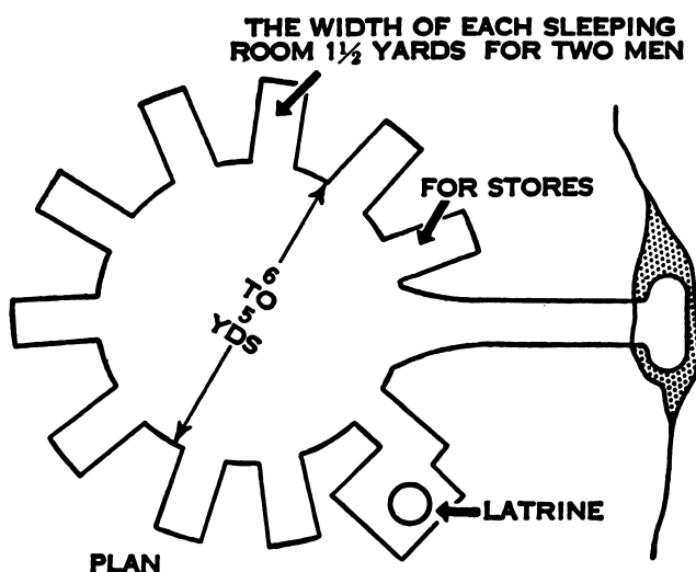
Figure 3-16. Snow cave for sixteen men.
