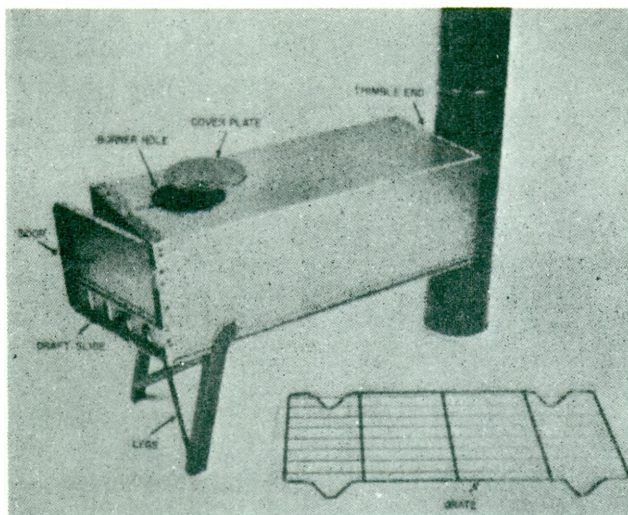
1 Body assembly
