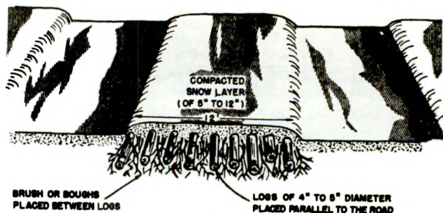
Figure 5-9. Road reinforced with brush, logs, and snow.
